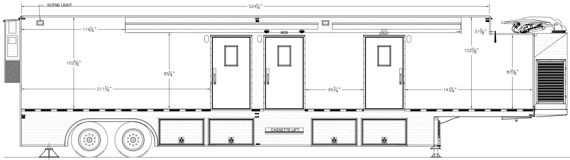
FRONT VIEW ELEVATION
