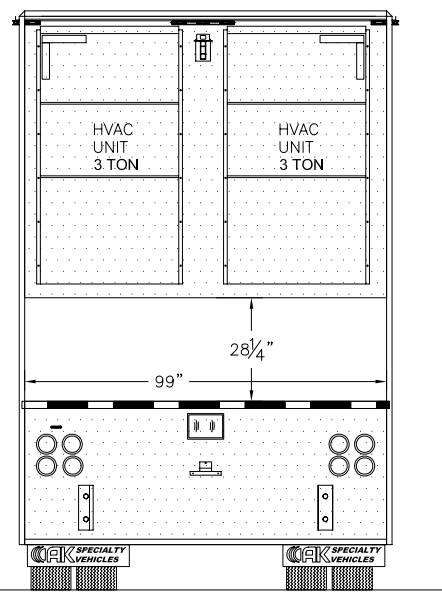
FRONT VIEW ELEVATION
